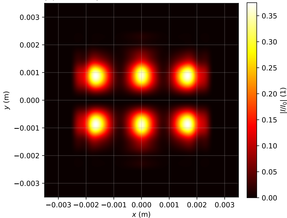
Intensity profile I(x, y, z = 3.662)/I_0 , P_{in}=3.0P_{cr} , artificial time
